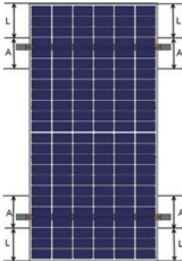
lamp zone: A = 200 mm
